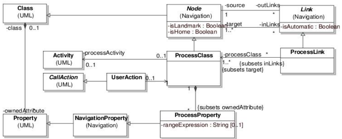
Figura 10 – UWE: Pacote de Processos (KROIB; KOCH , 2008)
